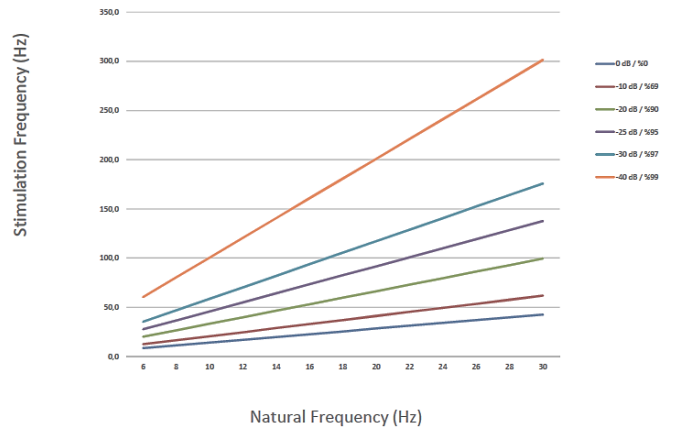
Vibration Isolation
