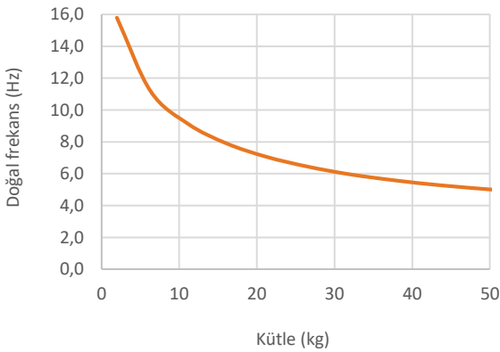
Kütle-Doğal Frekans (ASHRAE)
